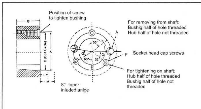
Dimensions for 3535 thru 5050 TAER Bushings
